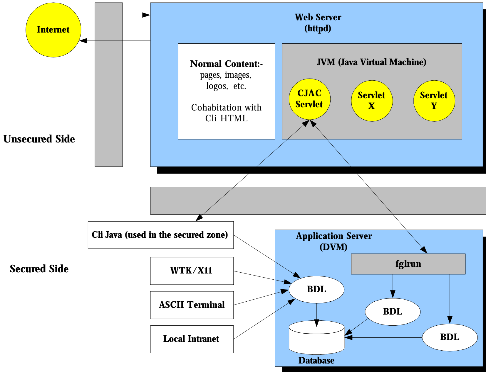
System Architecture for Java Client Deployment
